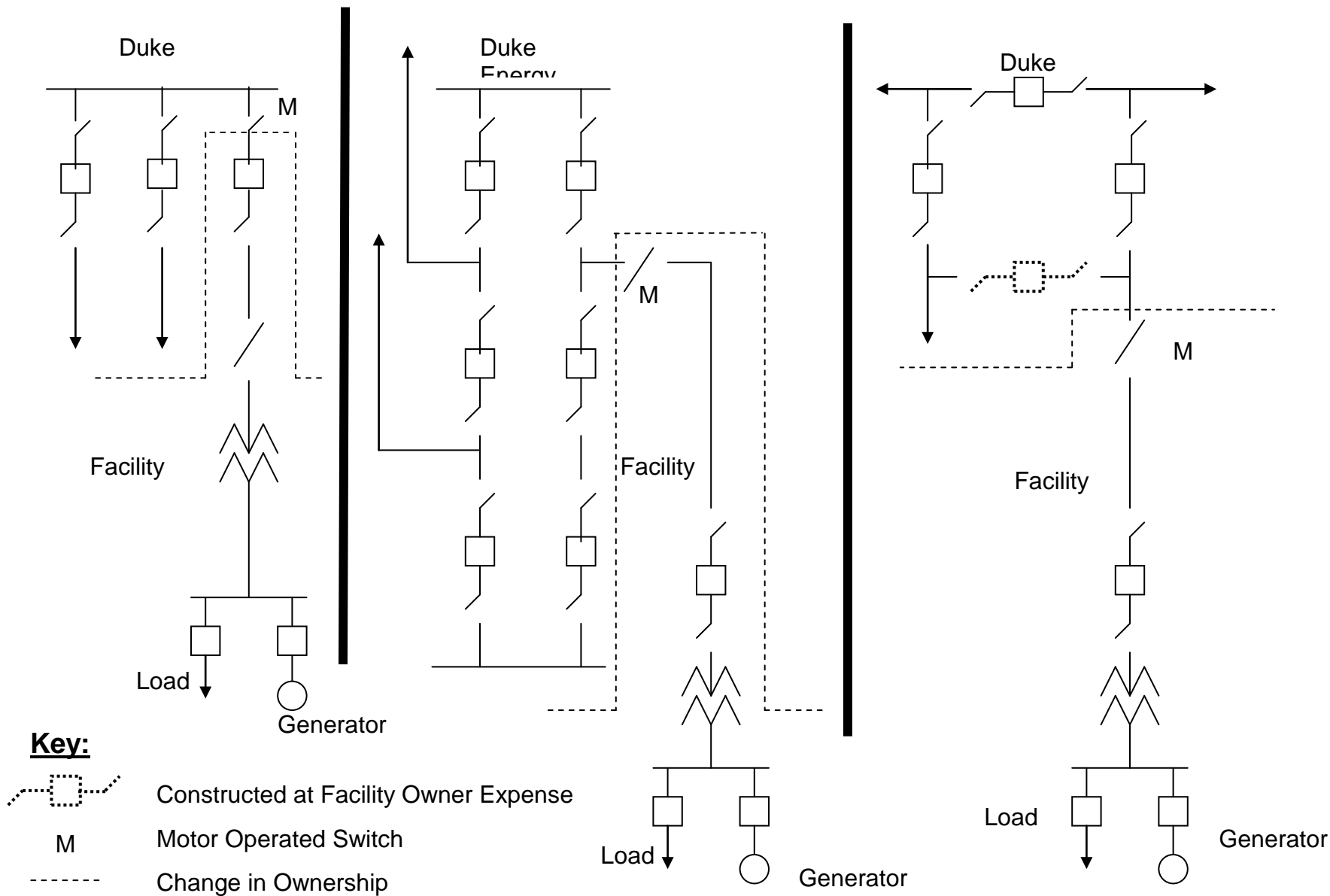
Figure 1 Typical Connection to Existing Substations
